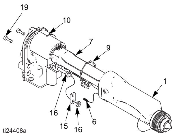
Fig. 35 . Barrel Installation
