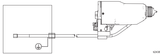
Fig. 10 Shielded Fluid Hose Connection at Non-Graco Isolation Enclosure
