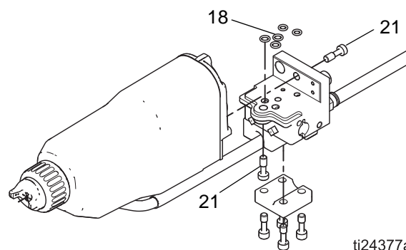
Fig. 27 Remove Gun from Manifold
