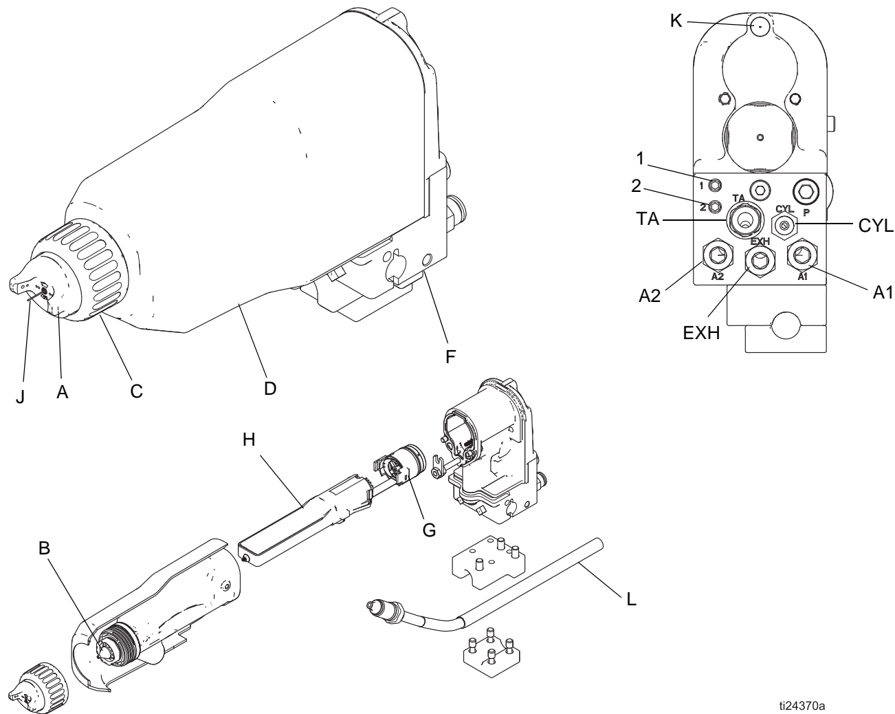
FIG. 2 . Gun Overview
