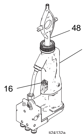
FIG. 30 . Fluid Packing Removal
