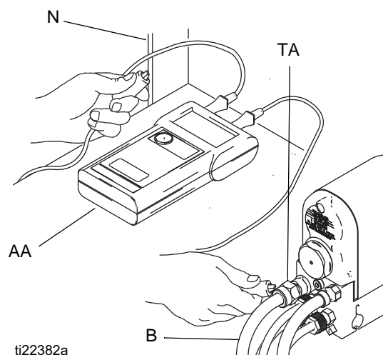
FIG. 15 . Check Gun Grounding
