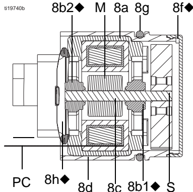
FIG. 39 . Turbine Cross-Section.
