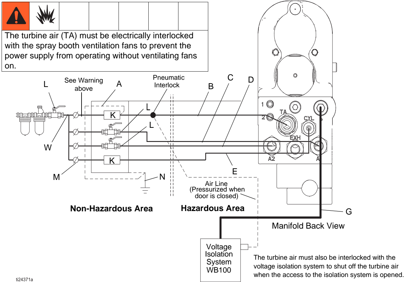
FIG. 3 . Typical Installation
