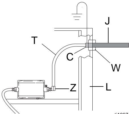
Fig. 9 Shielded Hose Connection at WB100 Enclosure
