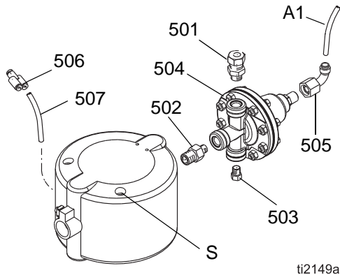
FIG. 14 . 245944 Fluid Regulator Kit
