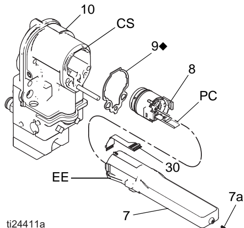
FIG. 37 . Power Supply
