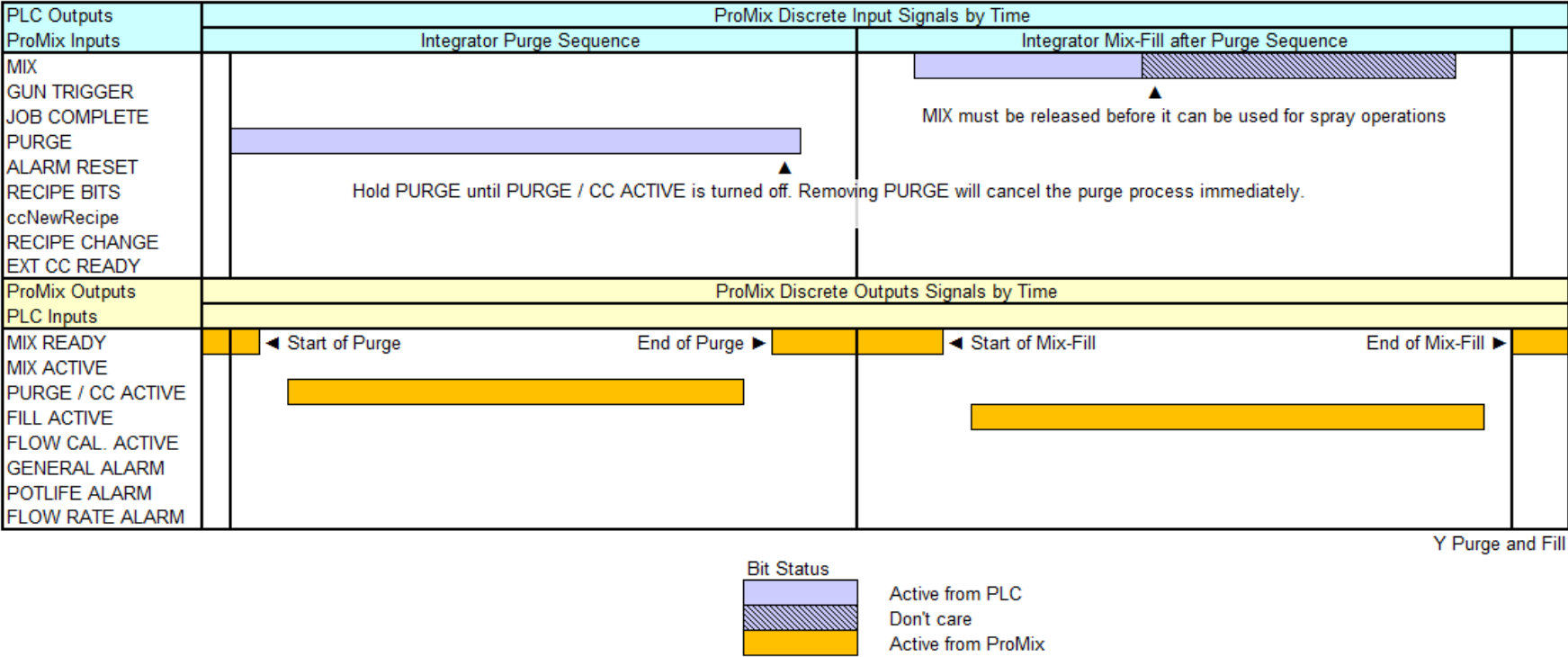
FIG. 81. Integration Control Y Purge and Fill
