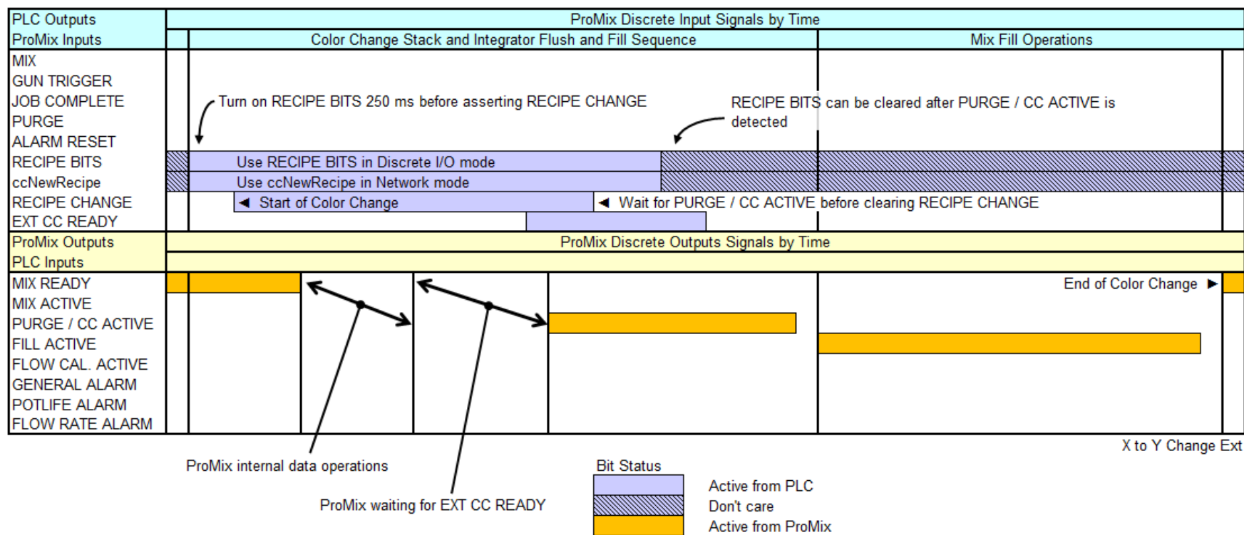
FIG. 78. Integration Control Recipe Change X to Y External Color Change
