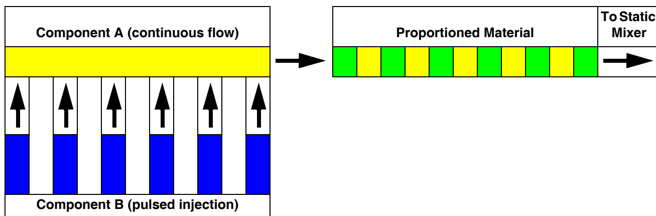
FIG. 105. Schematic Diagram of Dynamic Dosing Operation
