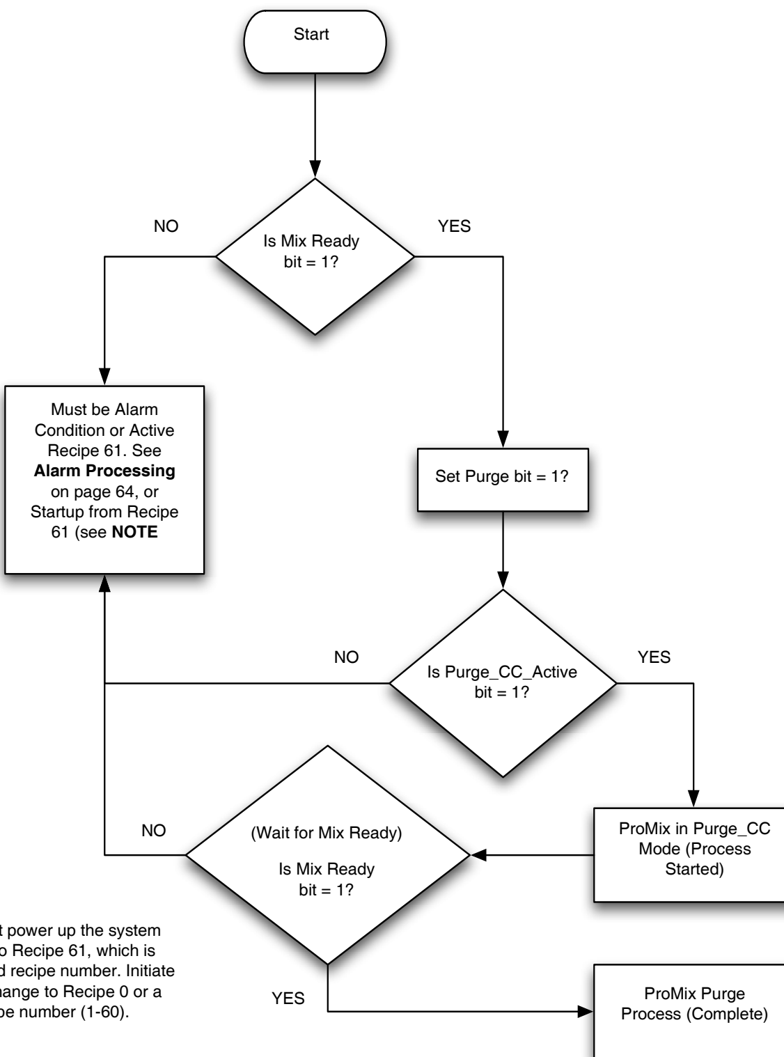
FIG. 73. Purge Mode Process Flow Chart
