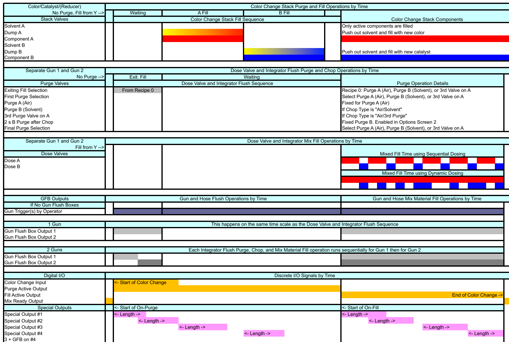
FIG. 124: ProMix 2KS Recipe Fill Chart #3 0 to Y
