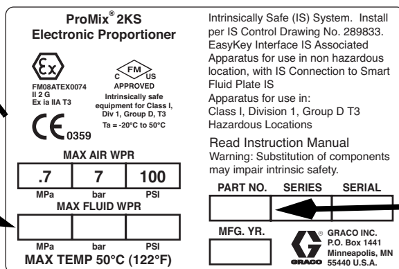
FIG. 1: Identification Label, Wall Mount Fluid Station Systems
