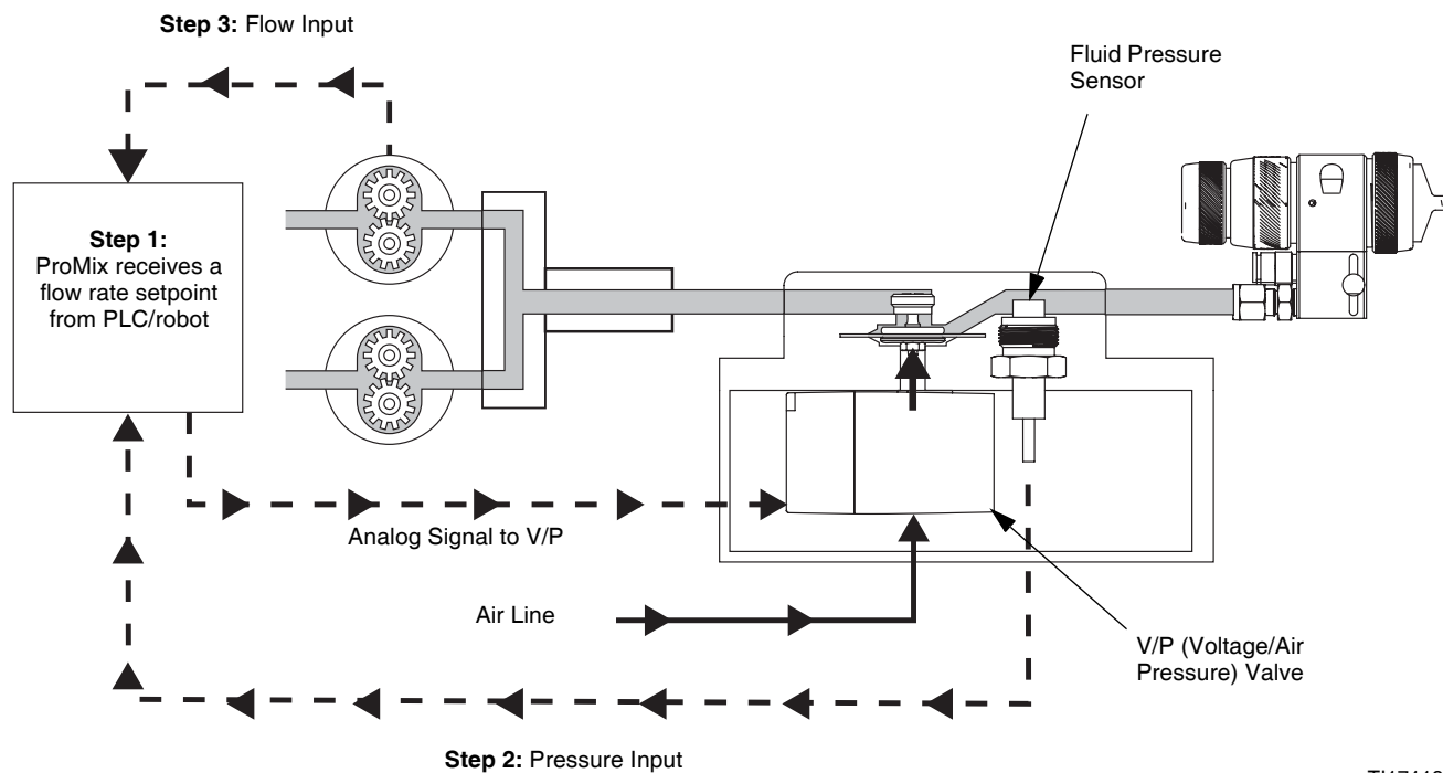
FIG. 88. ProMix Flow Control Pressure Loop and Flow Loop (249849 Module)
