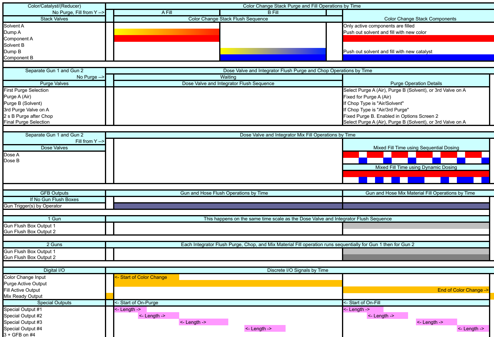
FIG. 125: ProMix 2KS Recipe Fill Chart #4 0 to Y
