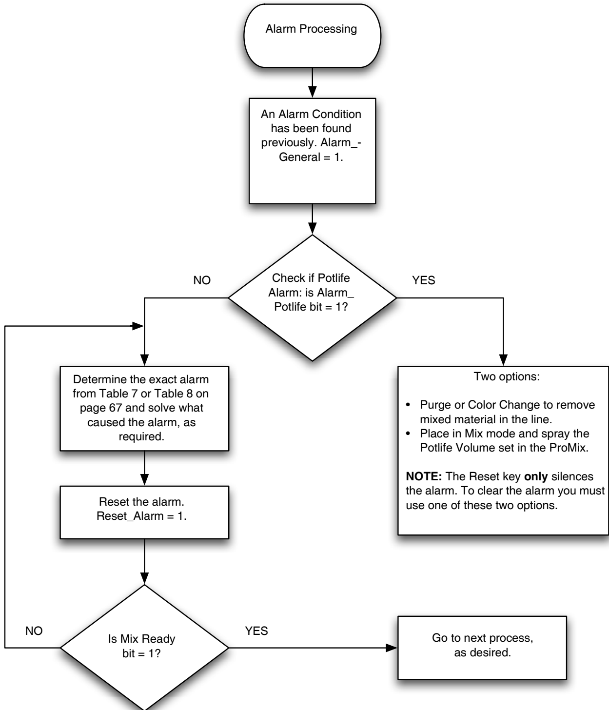
FIG. 75. Alarm Processing Flow Chart
