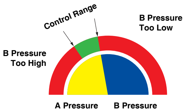
FIG. 110. A/B Control Range with Properly Sized Restrictor
