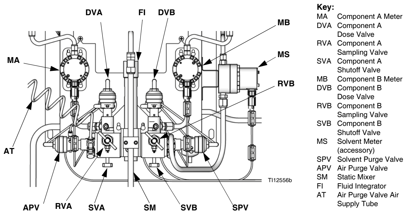
FIG. 119. Wall Mount Fluid Station
