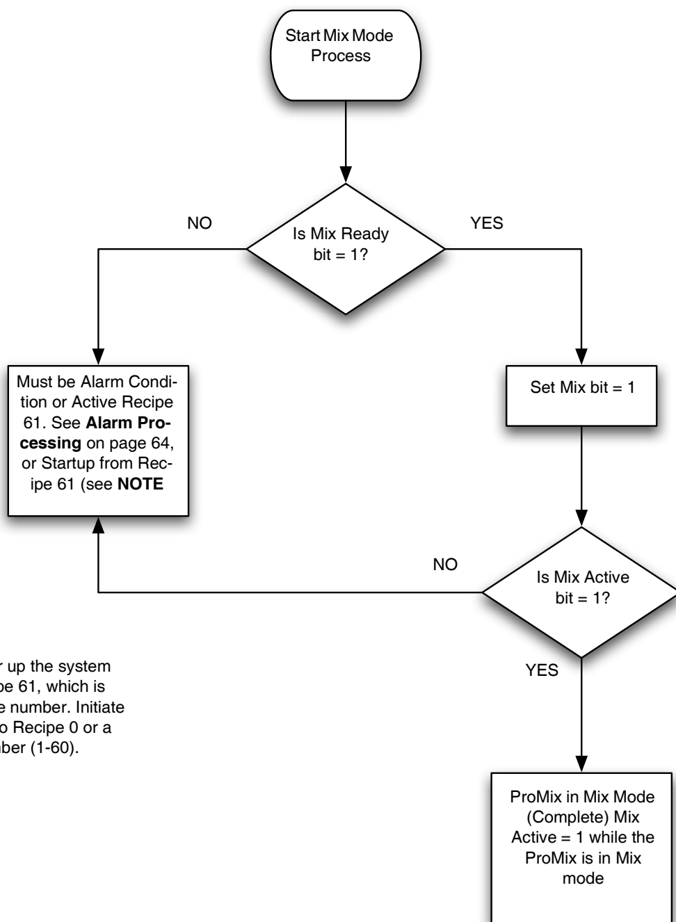
FIG. 71. Start Mix Mode Process Flow Chart
