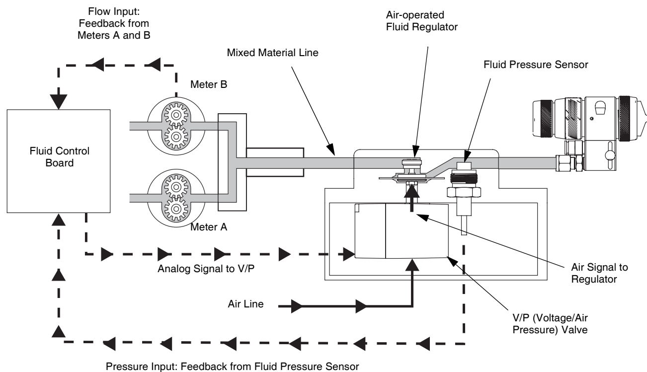
FIG. 86. ProMix Flow Control Schematic Diagram (249849 Module)
