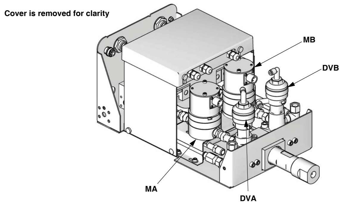
FIG. 6: Details of RoboMix Fluid Station
