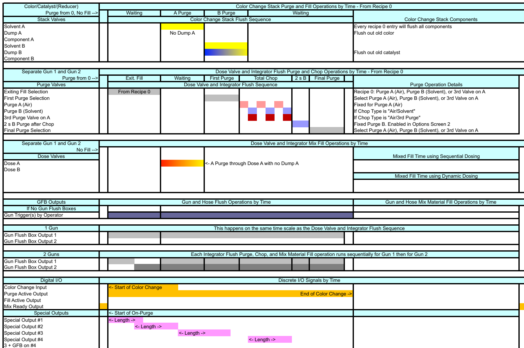
FIG. 131: ProMix 2KS Recipe Purge Chart #10 0 to 0
