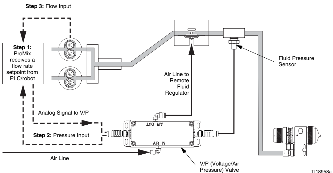
FIG. 89. ProMix Flow Control Pressure Loop and Flow Loop (24H989 Module)
