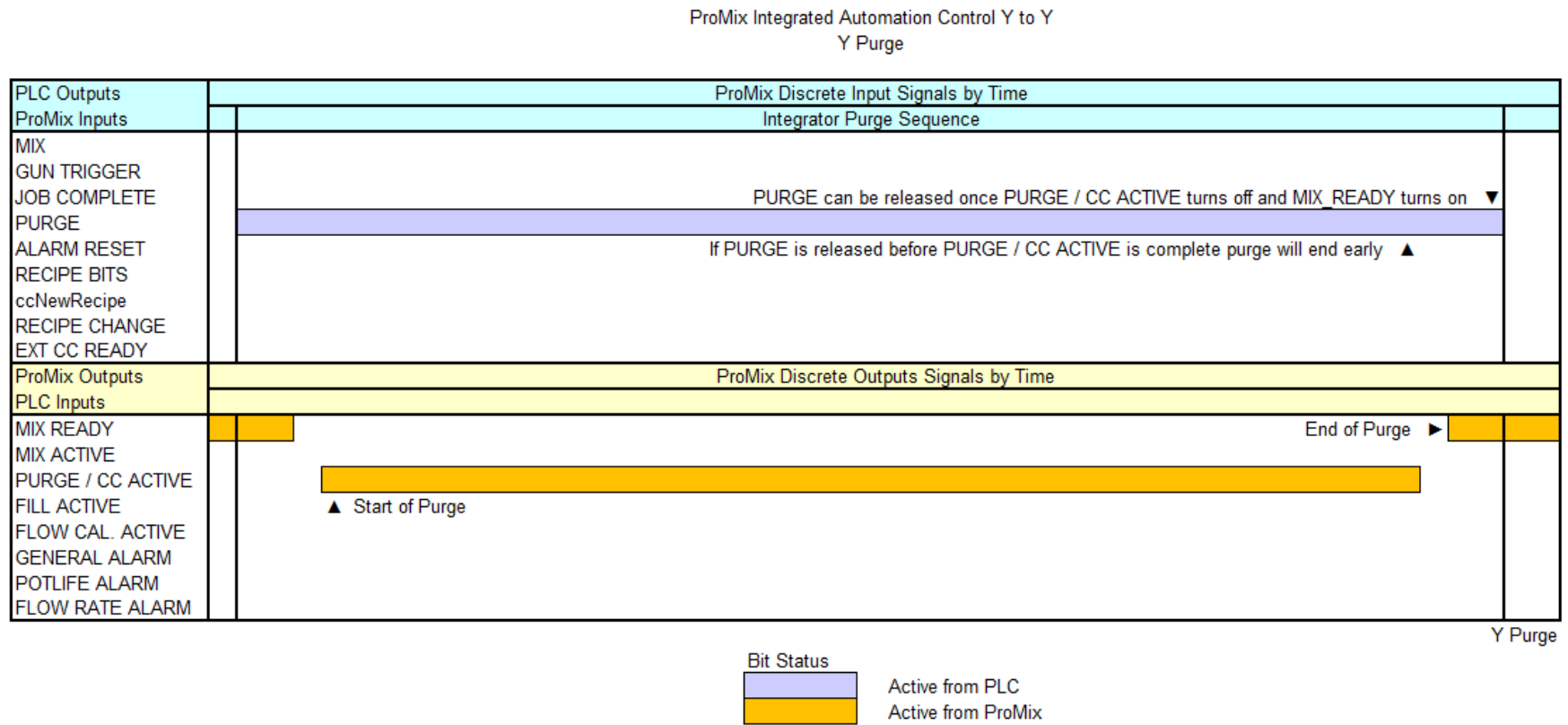
FIG. 79. Integration Control Y Purge
