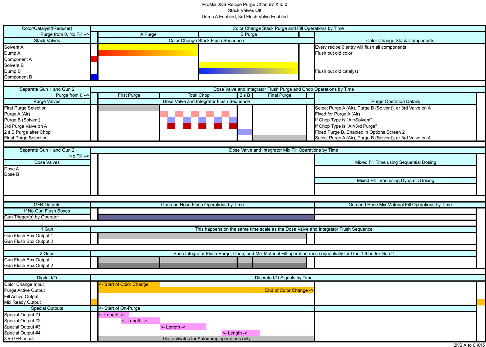
FIG. 128: ProMix 2KS Recipe Purge Chart #7 X to 0
