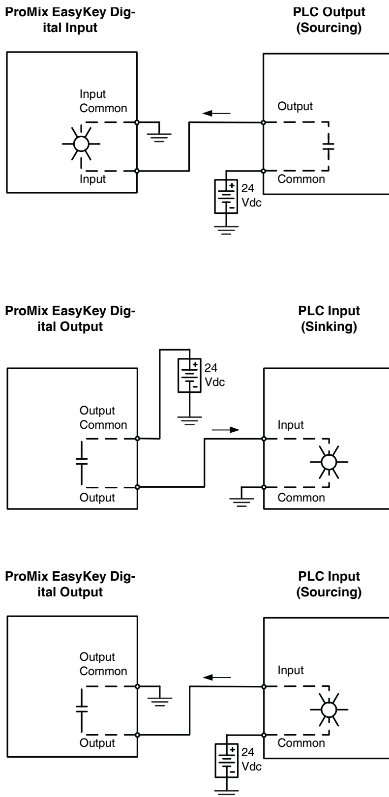
FIG. 76. Automation 24 Vdc Sourcing Input Diagram
