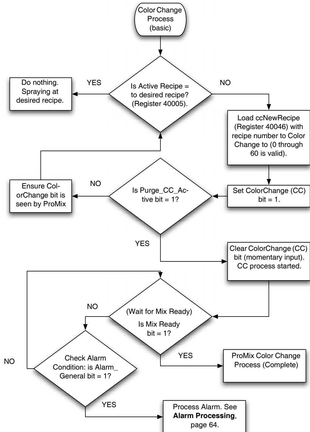
FIG. 74. Color Change Mode Process Flow Chart
