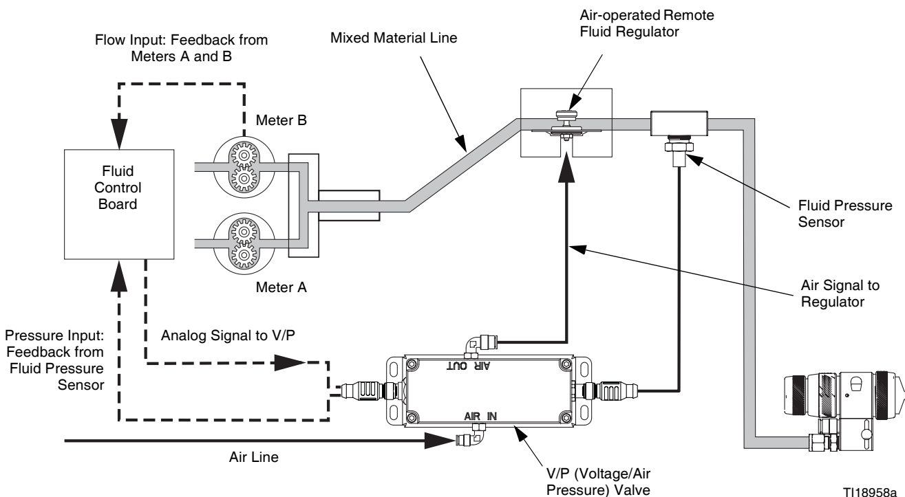
FIG. 87. ProMix Flow Control Schematic Diagram (24H989 Module)
