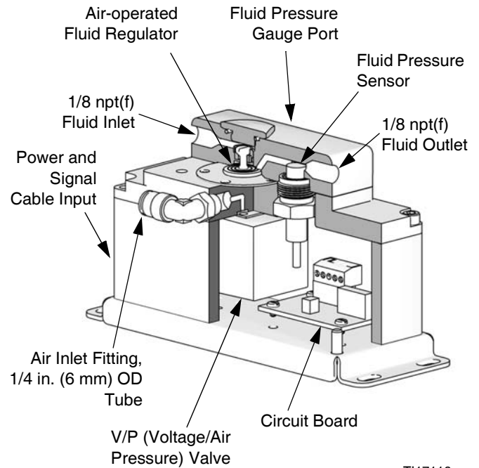
FIG. 84. Cutaway of 249849 Flow Control Module
