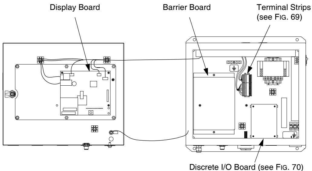
FIG. 68: EasyKey Control Boards
