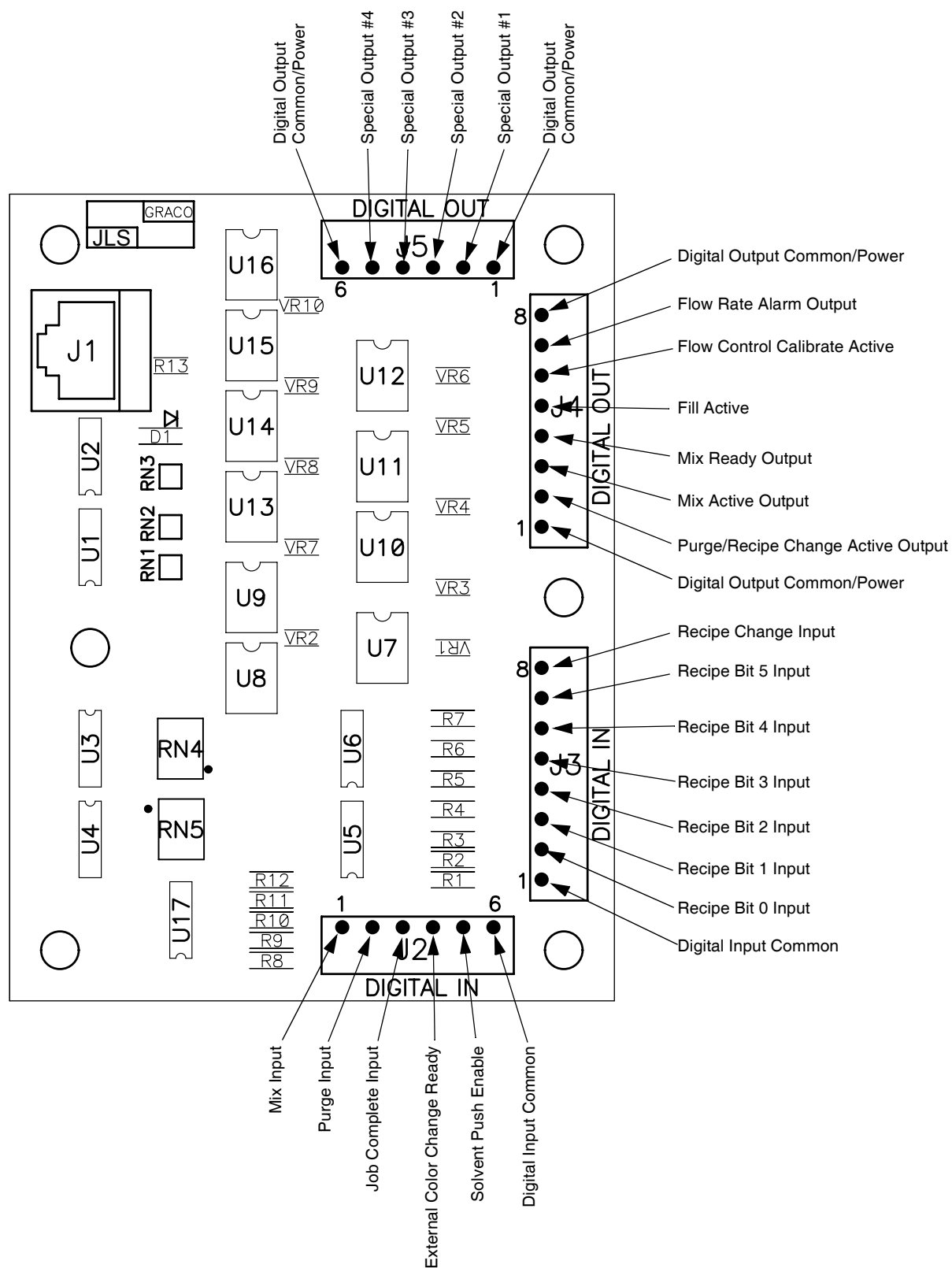
FIG. 70: 255766 Discrete I/O Board
