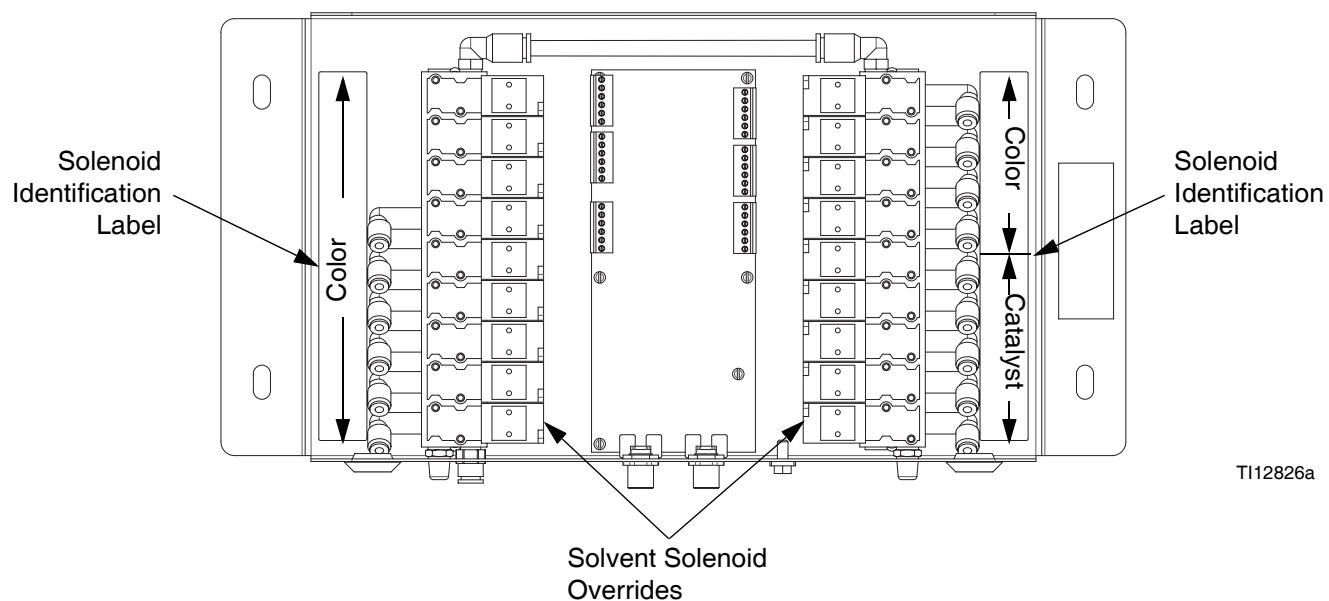
FIG. 118: Color Change Solenoids
