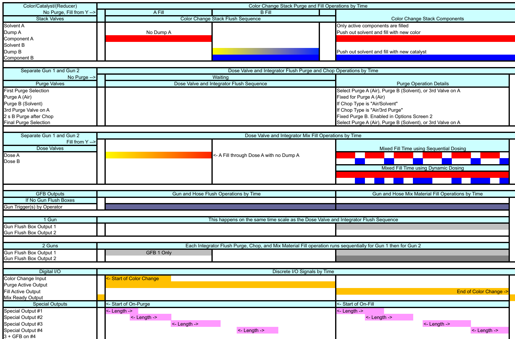
FIG. 127: ProMix 2KS Recipe Fill Chart #6 0 to Y
