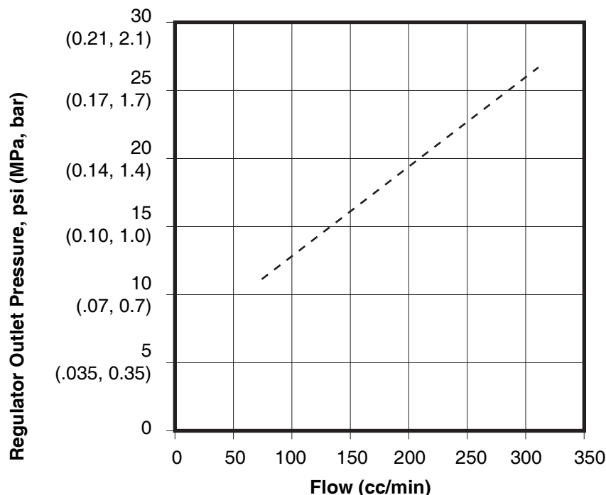
FIG. 99. Typical Flow Calibration (0-300 cc/min range)
