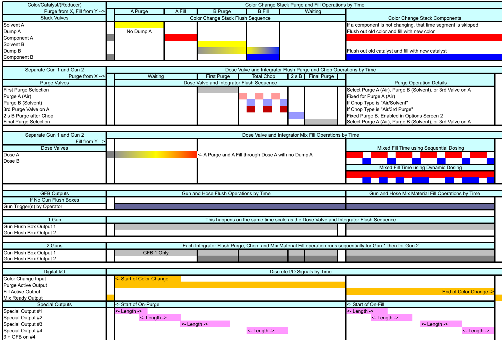
ProMix 2KS Recipe Change Chart #2 X to Y Stack Valves A1 to A2, B1 to B2 No Dump A, 3rd Flush Valve Enabled
