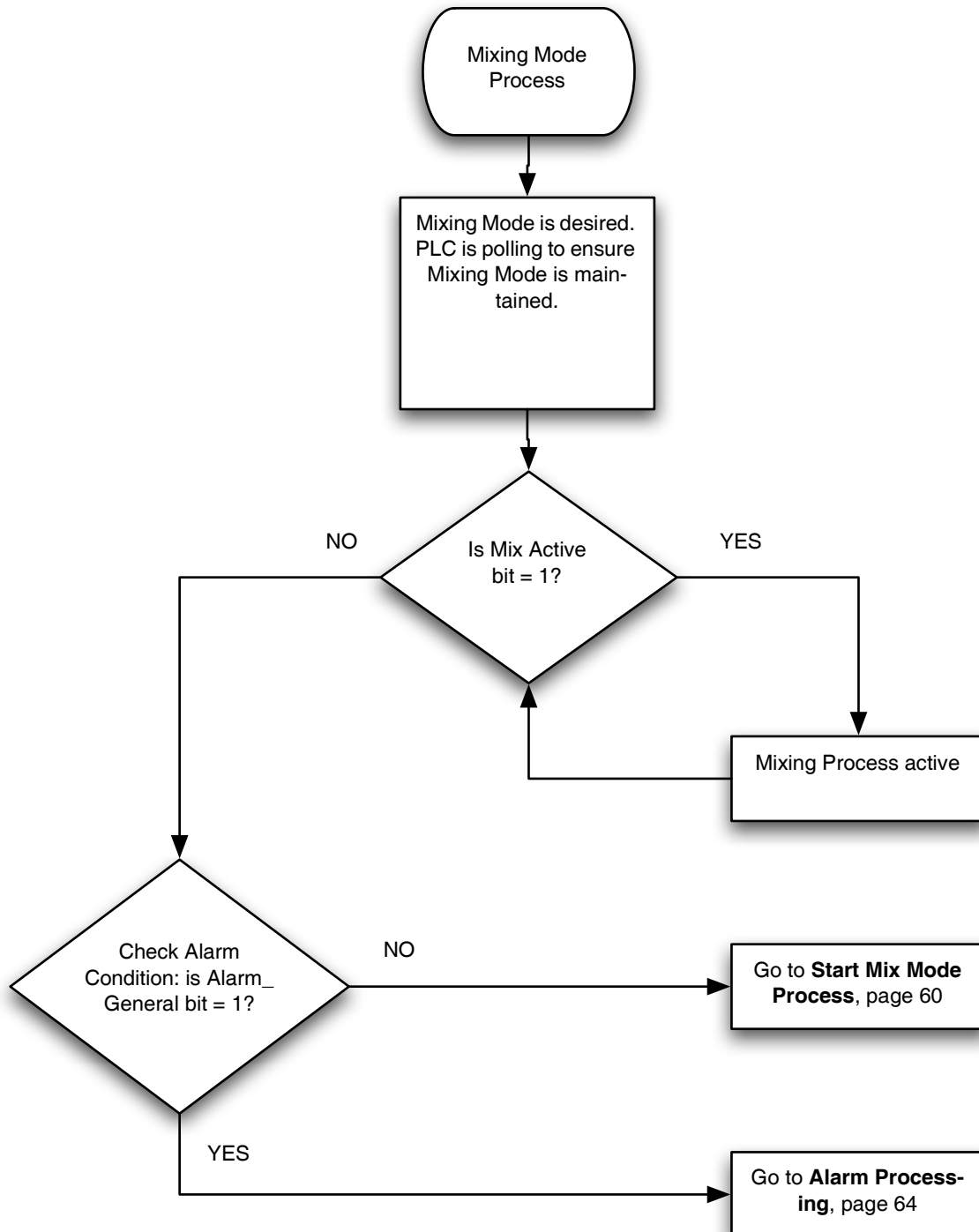
FIG. 72. Mixing Mode Process Flow Chart
