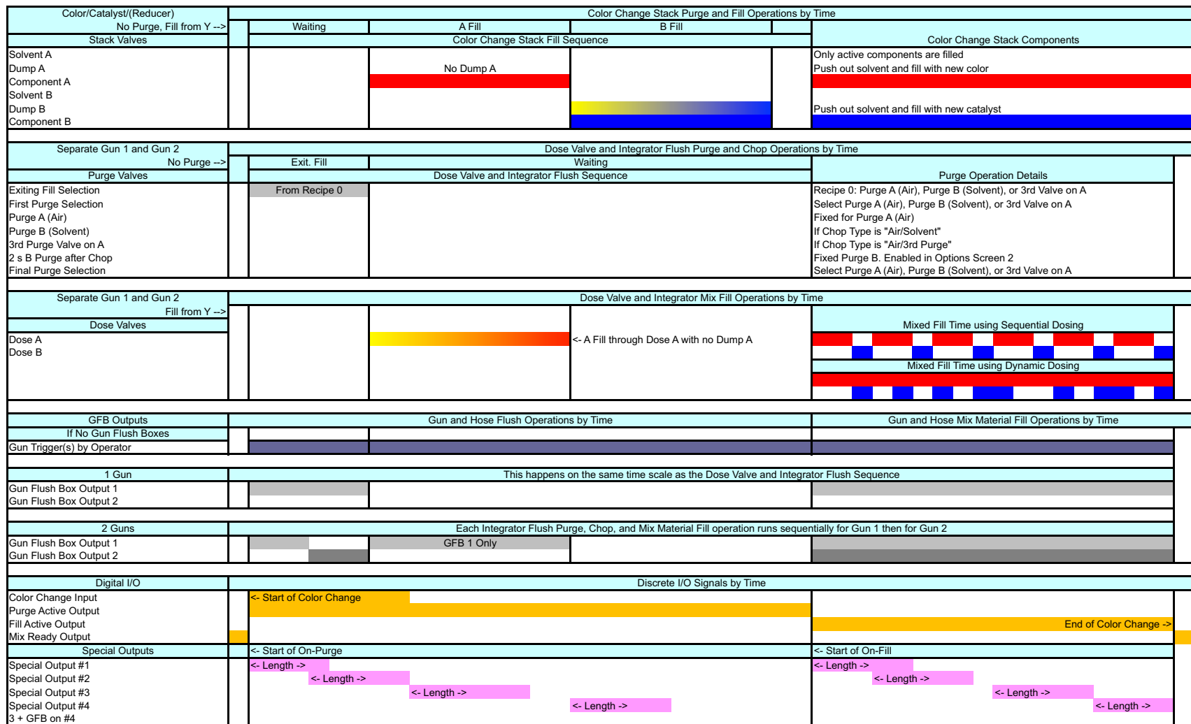
FIG. 126: ProMix 2KS Recipe Fill Chart #5 0 to Y
