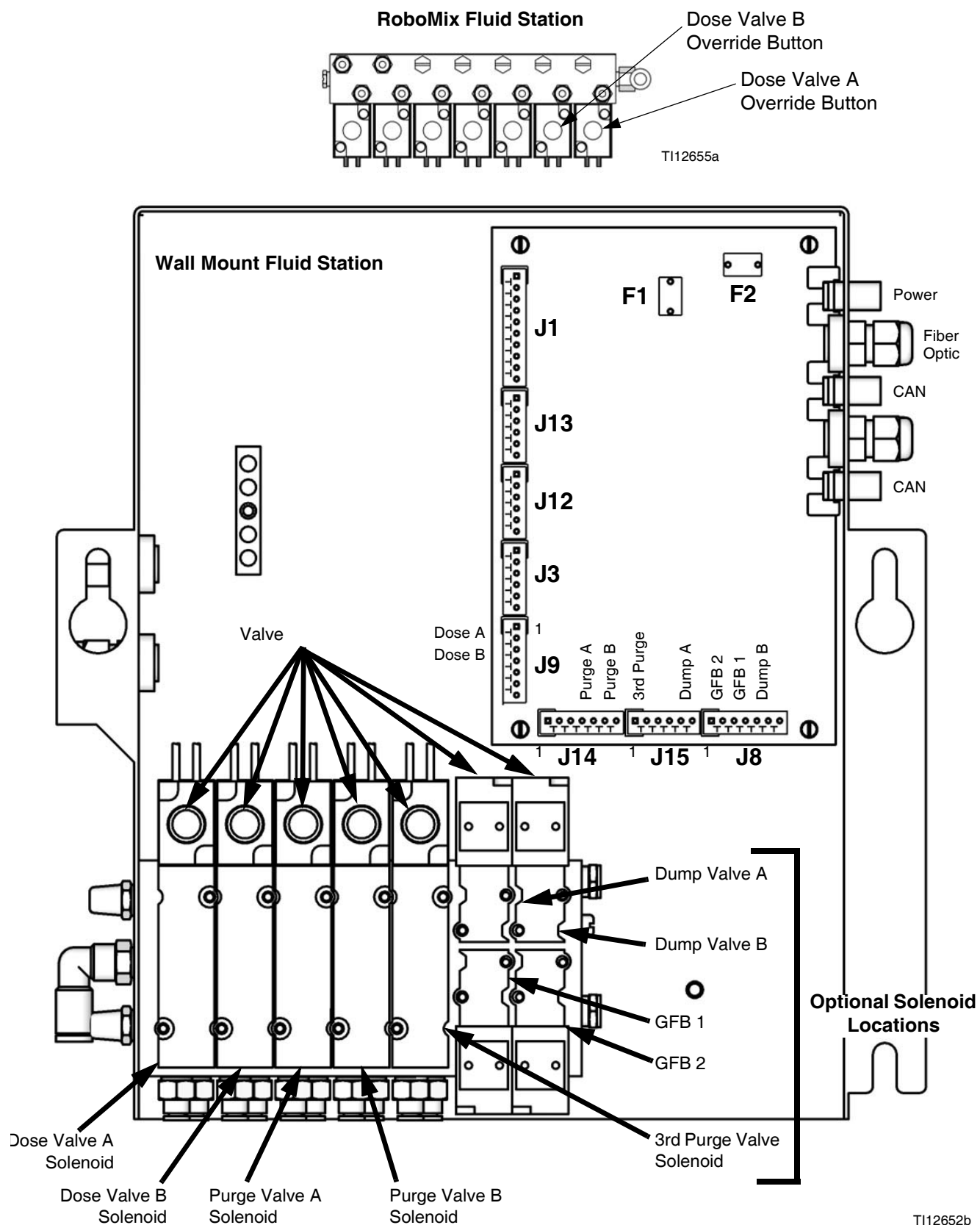
FIG. 117. Fluid Solenoids
