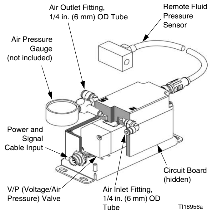
FIG. 85. Cutaway of 24H989 Flow Control Module
