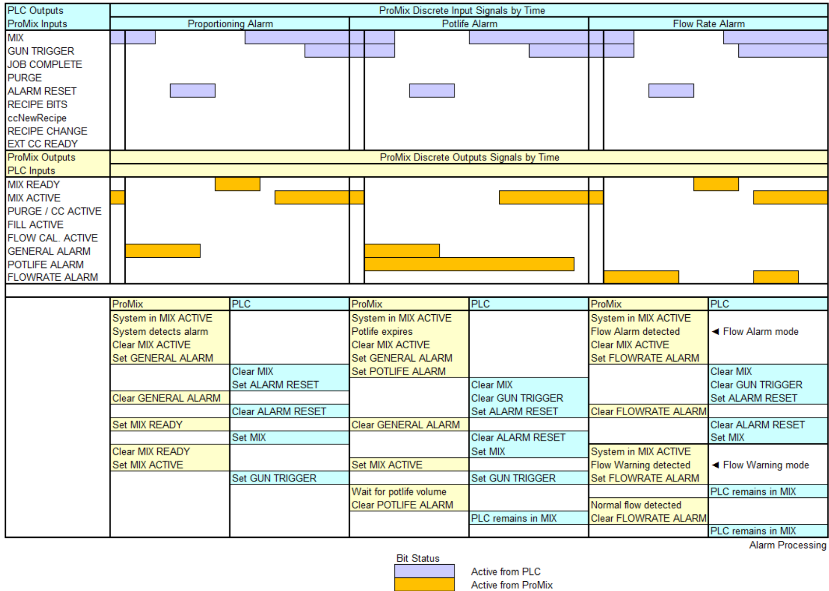
FIG. 83. Integration Control Alarm Processing
