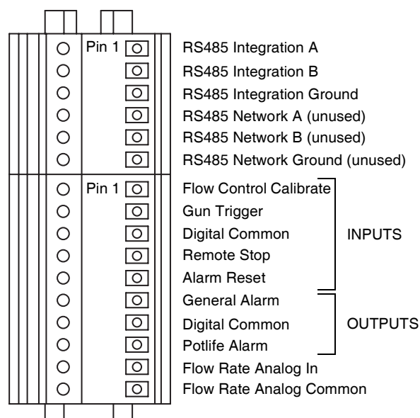
FIG. 69: EasyKey Terminal Strips
